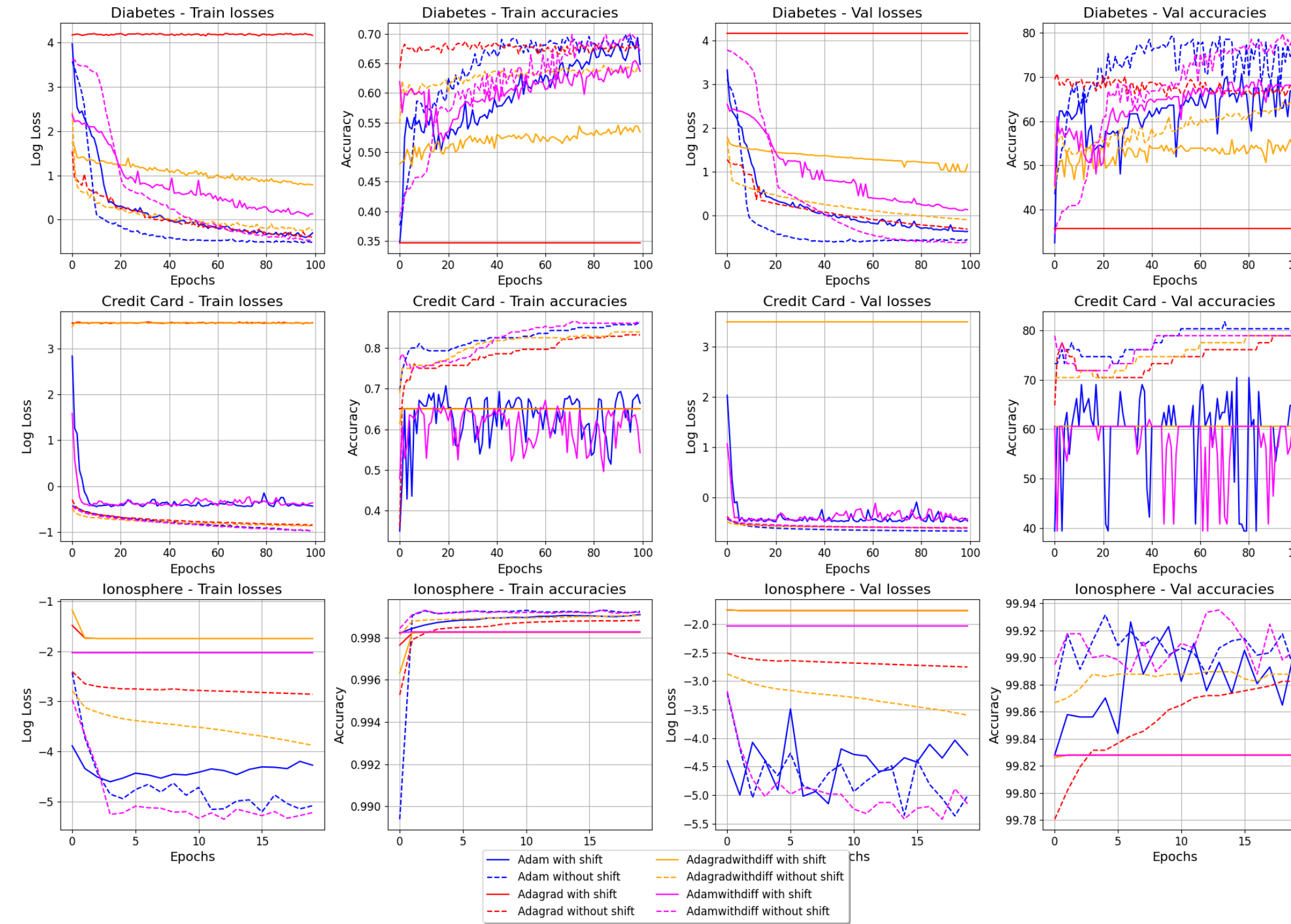
Figure 1. Comparison of losses and accuracies for different optimizers and data shifts on three datasets.
