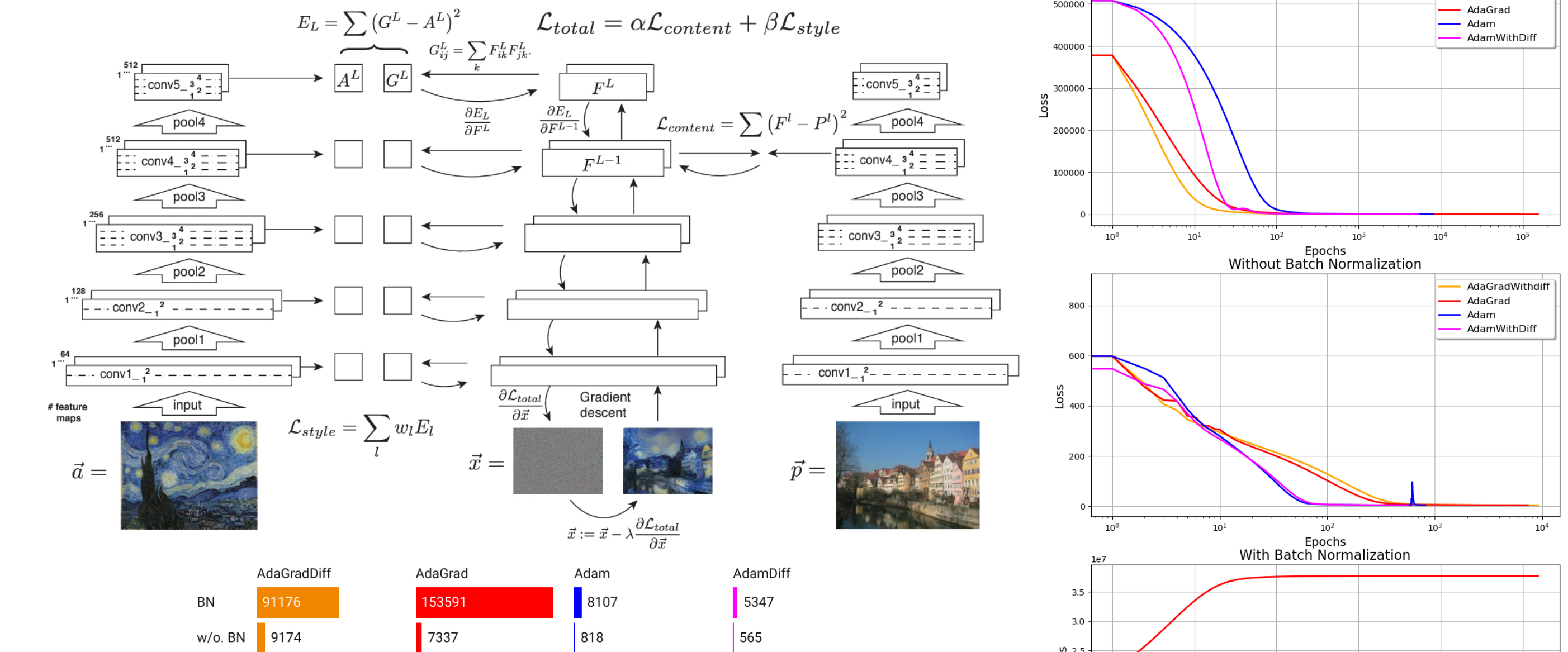
Figure 3. Epochs to converge to the given threshold. *The scales of epochs vary between models which is mainly due to the different settings of loss weights. The number of epochs is not necessarily the same with different parameter settings.
